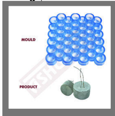
Round Cover Block Mould For Slab - 25MM (42 Cavity) Without Hole - 40mm Diameter
